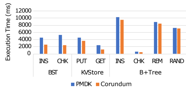
Figure 1: Performance comparison between Corundum and PMDK
